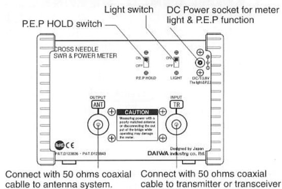
HP TYPE REAR PANEL
