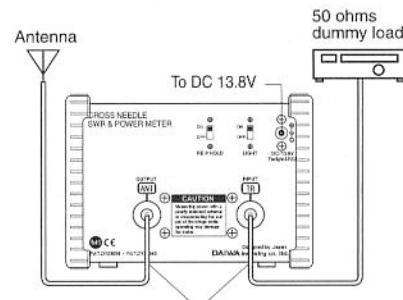
Fig. 1 50 ohms coaxial cable
