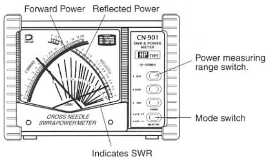
HP TYPE FRONT PANEL
